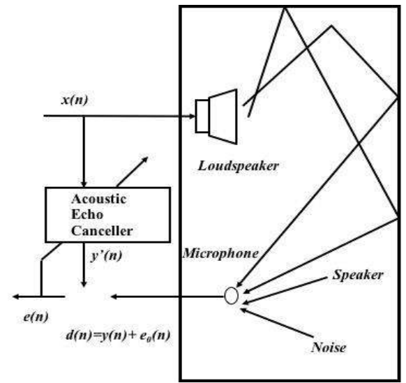
Fig. 1. Acoustic echo canceller.
