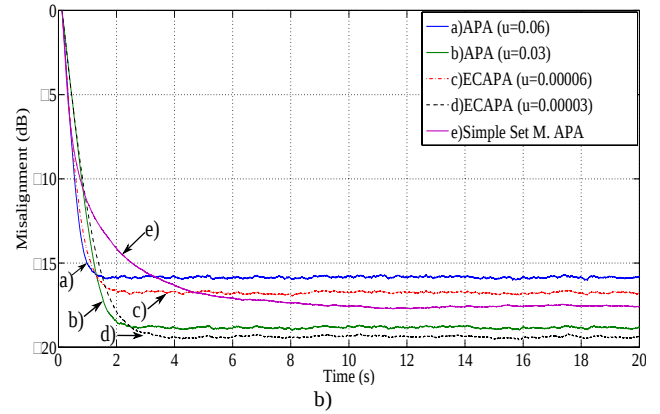
Fig. 4. a) Misalignment of the algorithms for K=5 , b) Misalignment of the algorithms for K=10 .
