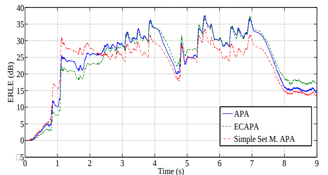
Fig. 2. ERLE curves for K=10 , the length of the adaptive filter is the same as the echo path and K=10 .
