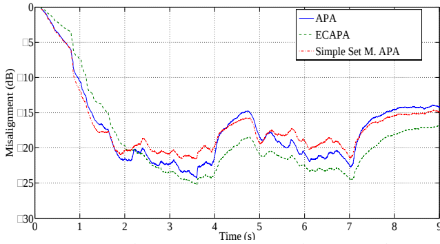
Fig. 3. Misalignment of the algorithms, the length of the adaptive filter is the same as the echo path and K=10 .
